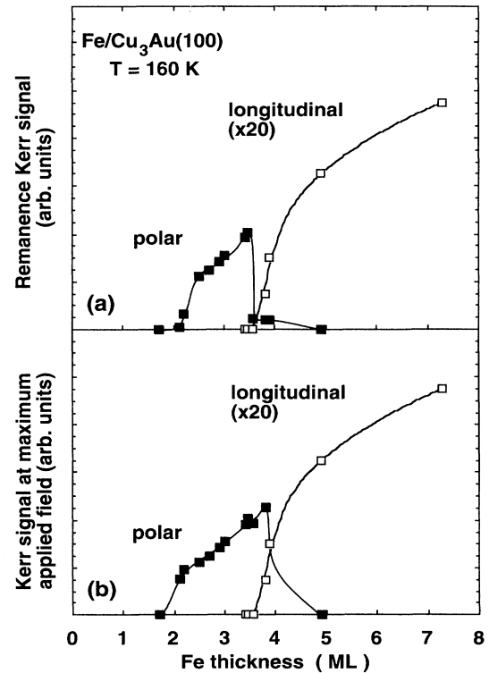
FIG. 6. Thickness dependence of the polar (filled squares) and longitudinal Kerr signal (open squares) at remanence (a) and maximum applied field (b) measured at T=160 K. Lines serve as a guide to the eye only.
