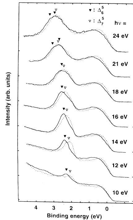
FIG. 2. Series of partial intensity spectra for different photon energies h\nu . Shown are spectra for the direction of the film magnetization and the light helicity parallel (solid lines) and antiparallel (dotted lines), calculated from the respective total intensity curves using an asymmetry corrected for the spin-filter efficiency of 0.22. Peak positions due to transitions from initial state bands containing \Delta_6^5 or \Delta_7^5 symmetry are indicated by solid and open triangles, respectively.
