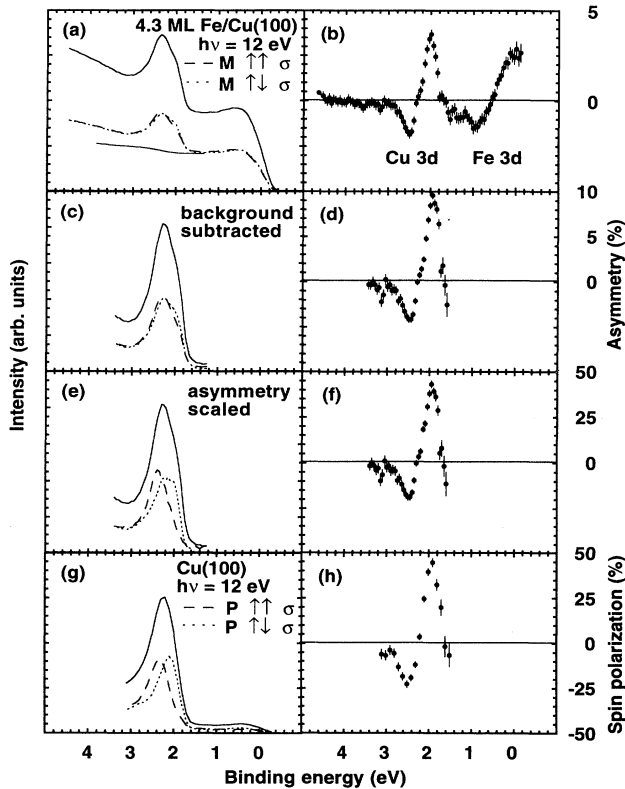
FIG. 1. (a) Photoelectron spectra of 4.3 ML Fe/Cu(100) at 12 eV photon energy for the direction of the film magnetization M parallel (dashed line) and antiparallel (dotted line) to the helicity \sigma of the exciting light, as well as the sum of both (solid line). (b) Asymmetry A , calculated from the spectra of (a) using the formula A = [I(\uparrow\downarrow) - I(\uparrow\uparrow)]/[I(\uparrow\downarrow) + I(\uparrow\uparrow)] . (c) Same as (a), but in the region of the Cu 3d peak corrected for the background induced by the Fe 3d emission as indicated in (a). (d) Asymmetry, calculated from the spectra of (c). (e) Total intensity curve (solid line) identical to the one in (c), partial intensities calculated from an asymmetry which is scaled by 1/S ( S = 0.22 , spin-filter efficiency) with respect to the one shown in (d). (f) Asymmetry corresponding to the spectra of (e). (g) Spin-resolved photoelectron spectra of clean Cu(100) at 12 eV photon energy. Given are the spectra for the vectors of the electron spin polarization P and the light helicity \sigma parallel (dashed line) and antiparallel (dotted line) as well as the spin integrated spectrum (solid line). (h) Spin polarization P , calculated from the spectra of (g) using the formula P = [I(\uparrow\downarrow) - I(\uparrow\uparrow)]/[I(\uparrow\downarrow) + I(\uparrow\uparrow)] .
