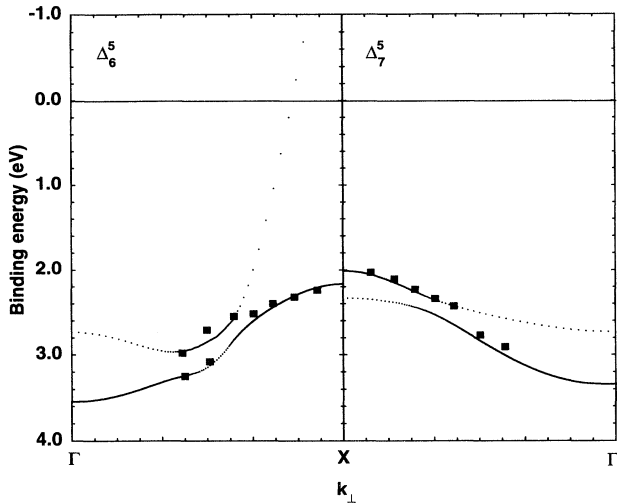
FIG. 3. Relativistically calculated band structure of copper along the \Delta axis (dotted lines, from Ref. 21), together with the experimentally observed spin-resolved photoemission peaks from Fig. 2. Left: bands containing portions of \Delta_6^5 symmetry and experimental peak positions for spin polarization parallel to the light helicity. Right: bands containing portions of \Delta_7^5 symmetry and experimental peak positions for spin polarization antiparallel to the light helicity. The portions of \Delta_6^5 and \Delta_7^5 symmetry are indicated by the density of the dotted lines.
